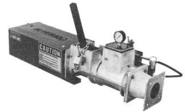
MODEL 440 VACUUM DEAIRING PUGMILL 350 Pounds per Hour
